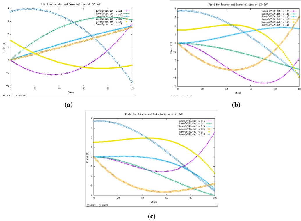
Figure 3: plots of the Field trajectory during the Rotator Ramp for 41, 100 and 275 GeV
