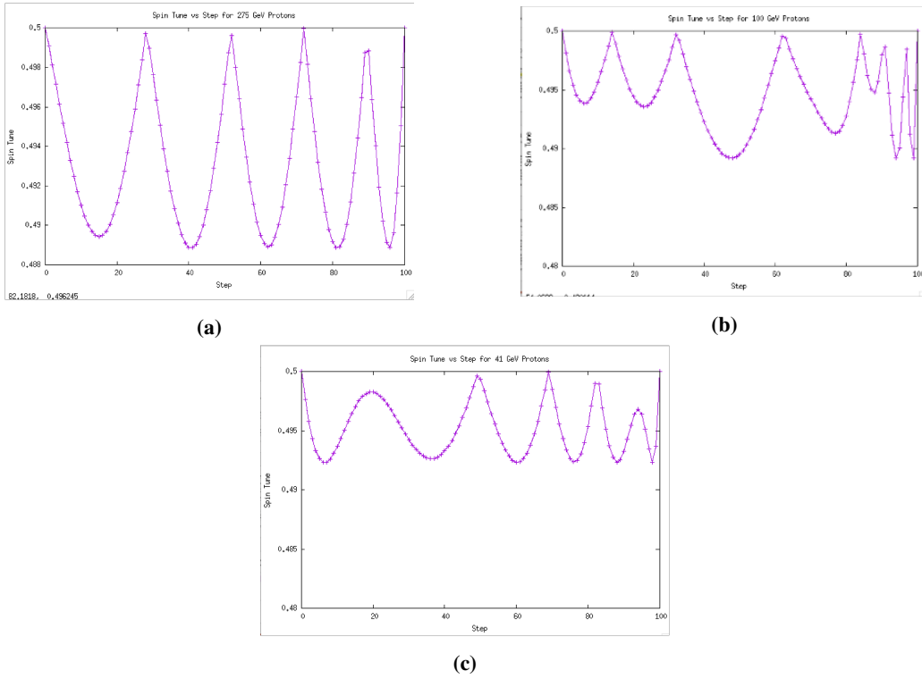
Figure 2: plots of Spin tune during the Rotator Ramp for 41, 100 and 275 GeV
