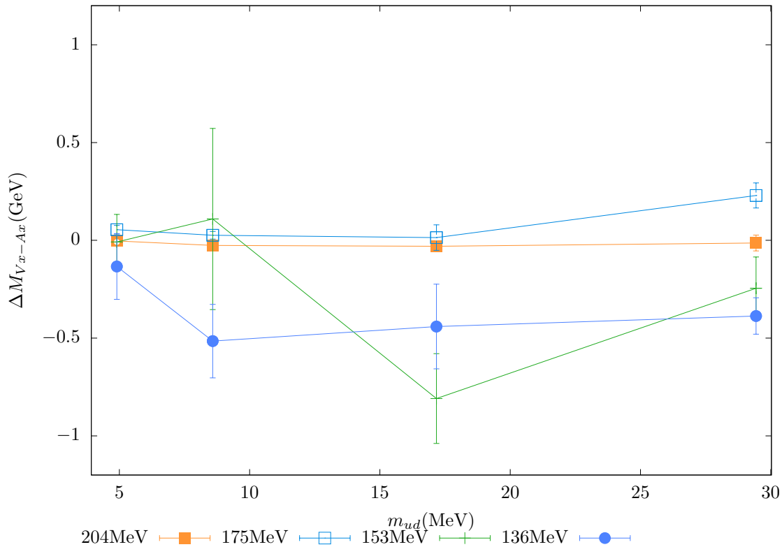
SU(2)_L \times SU(2)_R Symmetry Plot : V_x - A_x Screening Mass Difference
