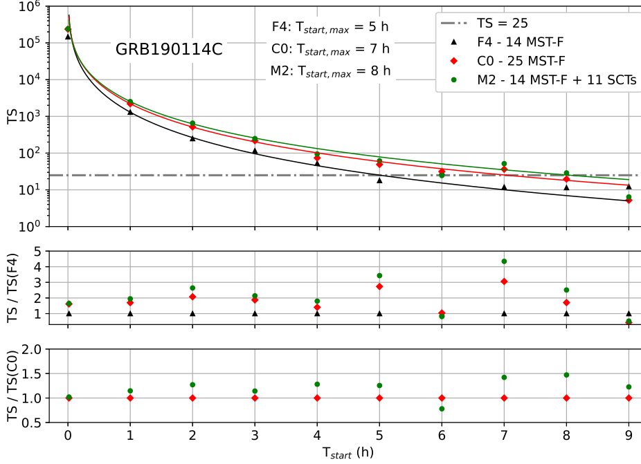
Figure 3: In the top panel, TS values resulting from the analyses of 1-hour GRB 190114C observations at different T_{start} , from T_0 + 60 s, for the three layouts of interest. In the mid and bottom panels the TS values normalized to F4 and C0, respectively.
