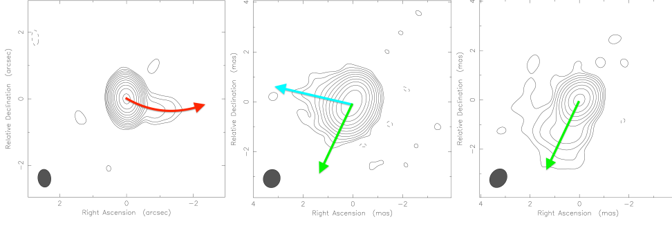
Figure 2: Left: The jet of J1048+7143 as seen at 4.8-GHz with the VLA. The jet is oriented towards west and it extends to \sim 15 kpc projected distance (red arrow). Middle and right: Two examples of the 8.6-GHz jet structure observed with the VLBI (observing dates 2001 Jul 7 and 2010 Mar 23, respectively). In the mas-scale structure (8.361 pc/mas), there is an approximately eastern (turquoise arrow) and a southern jet extension (green arrow), such that sometimes the eastern and sometimes the southern jet dominates.
