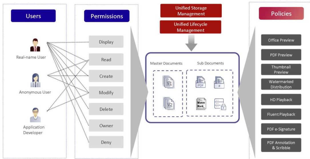
Figure 8 Permission management of IHEP Docs
