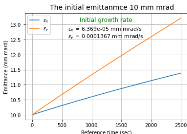
Figure 5: Emittance growth for a lattice with \beta_{y-max} = 33 m vs time. The beam interacts with residual gas only. The initial Horizontal and Vertical emittance growth rates ( \epsilon_x, \epsilon_y ) are also shown within the plot.
