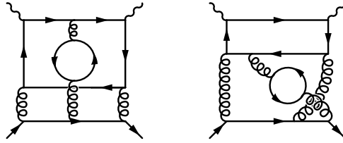
Figure 1: Some of the most complicated diagrams contributing to the computation for the n_f^2 third-order coefficient functions for F_{3,ns} . All diagrams come with the color factor n_f^2 d^{abc} d_{abc} / n_c . When computing the boundary conditions, the first and second diagram will correspond to the BE and O4 topology in MINICER notation [34, 35] with a bubble insertion, respectively.
