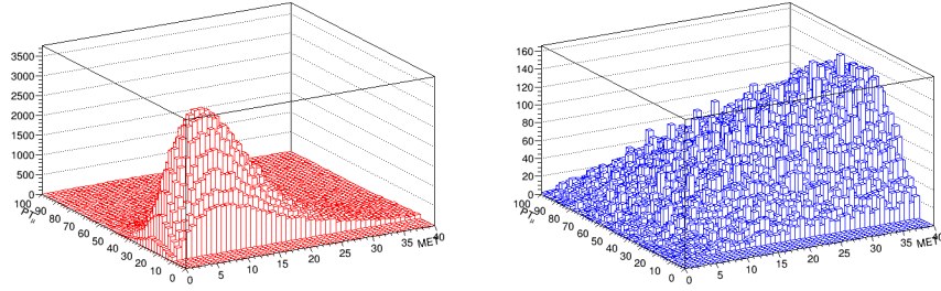
Figure 3: Correlation between p_T^H vs. E_T for the signal (red) and background (blue) at detector level
