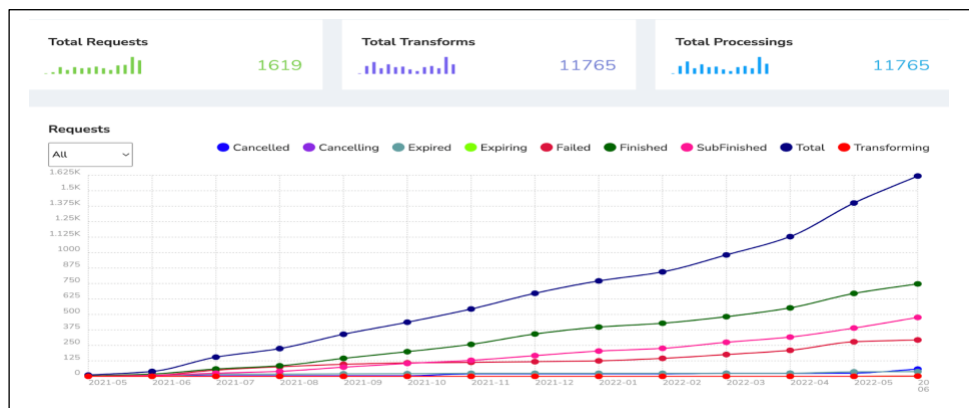
Fig. 3. Since late 2021 in Rubin Observatory, iDDS-PanDA within the LSST framework has processed more than 11000 tasks, where many tasks have more than 10K jobs.
