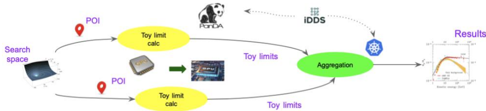
Fig. 7. Multiple-steps Monte Carlo Toy based confidence limits calculations and aggregations.
