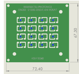
Figure 2: SiPM panel
