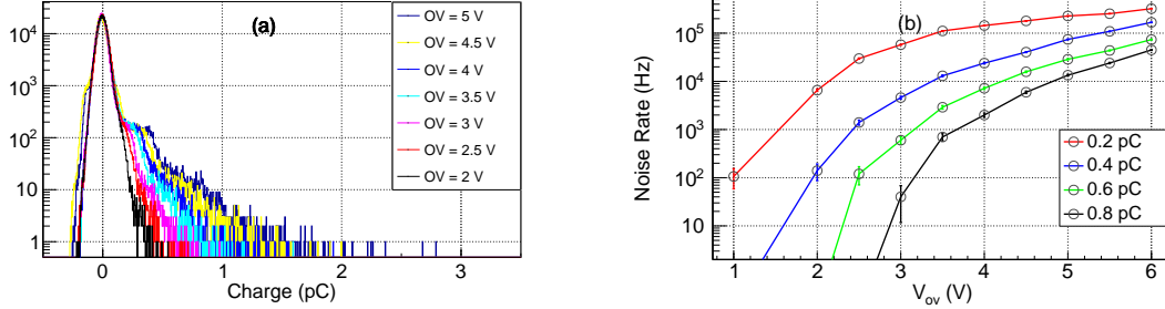
Figure 7: (a) The integrated charge distribution from the noise data at different V_{ov} and (b) Variation in the noise rate at different q_{th} for different V_{ov}
