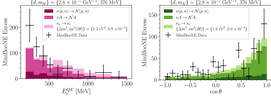
Figure 1: E_\nu^{QE} (left) and \cos \theta (right) distributions of the MiniBooNE excess for a representative point of the 3 + 1 + \mathcal{N} -decay model. The error bars on the energy distribution include systematic and statistical errors, while for the angular distribution only statistical errors are included. Taken from [10].
