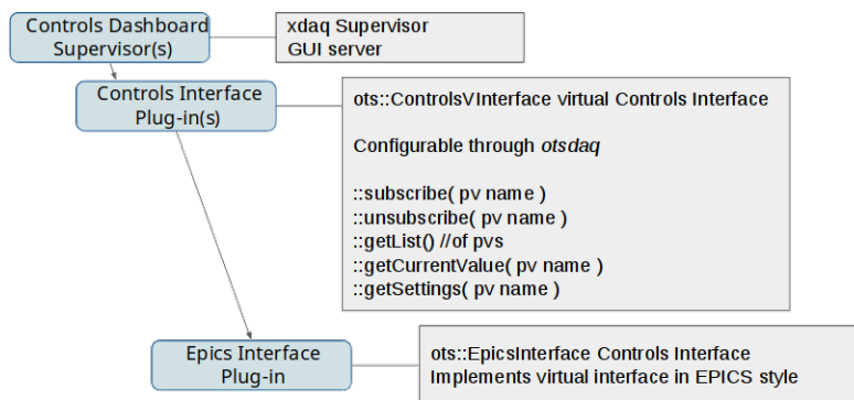
Figure 2: otsdaq C++ classes designed for EPICS interfacing.
