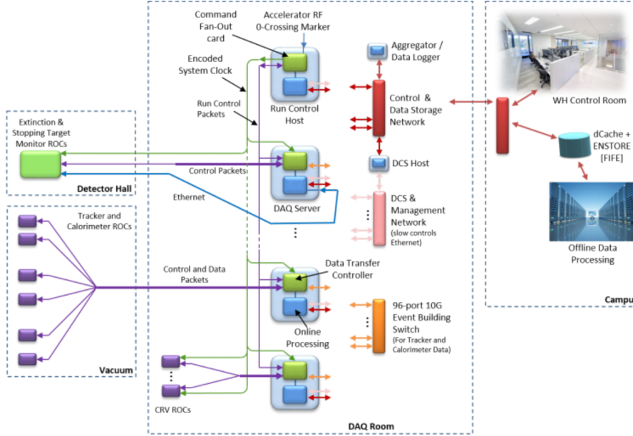
Figure 1: Mu2e TDAQ architecture and components diagram.
