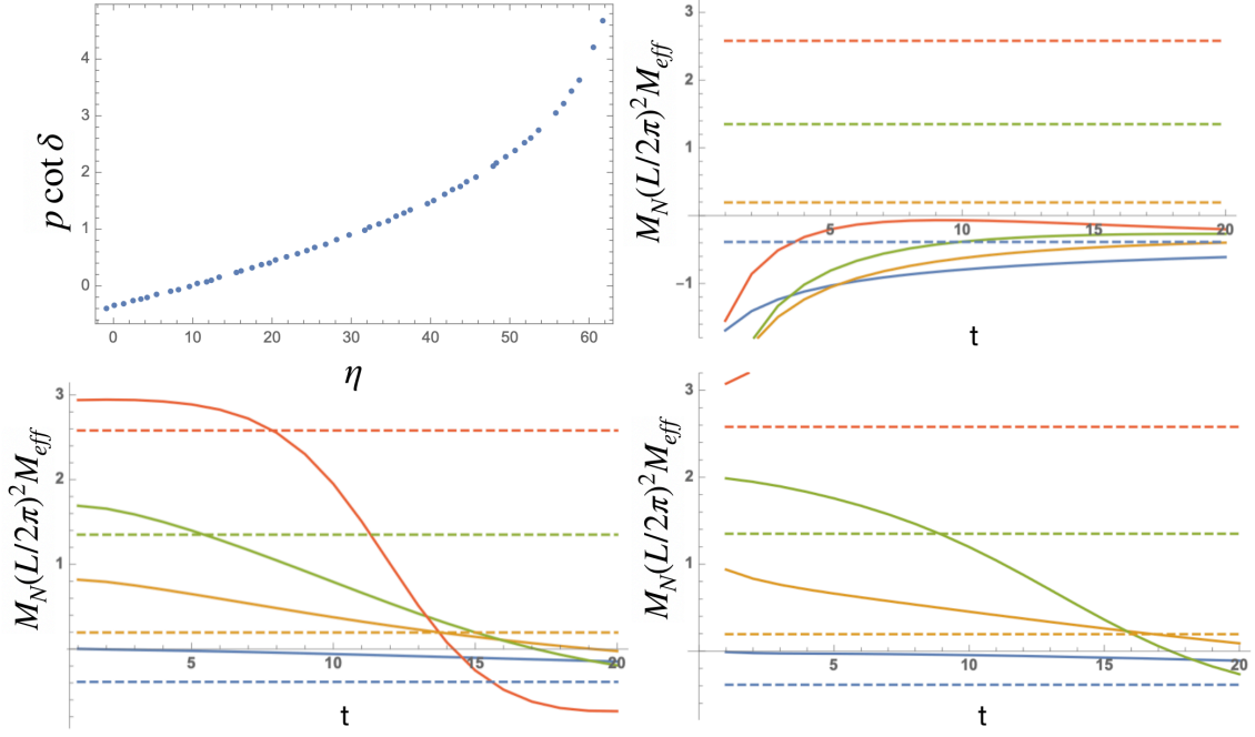
Figure 5: Upper left: Scattering phase shift in lattice units versus momentum, \eta = \left(\frac{pL}{2\pi}\right)^2 for the second system discussed in Sec. 3.2, having a deeply-bound ground state. Upper right: Effective masses for the two-nucleon system in an L = 12 box using local hexaquark two-nucleon operators at the source and momentum-space operators at the sink. Lower panels: Effective masses for the two-nucleon system in an L = 12 box using two-nucleon operators spatially displaced by \Delta = 1 (left) and \Delta = 5 (right) at the source and momentum space operators at the sink. The exact spectrum in these panels is shown as a set of dashed lines.
