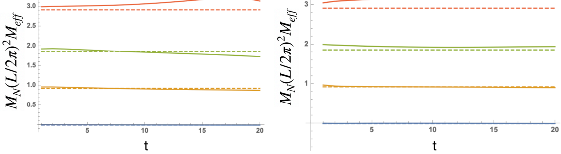
Figure 4: Effective masses for the two-nucleon system for the scattering phase shift shown in Fig. 1 (no physical bound state) using two-nucleon operators spatially displaced by \Delta = 1 (left) and \Delta = 5 (right) at the source and momentum space operators at the sink. The exact spectrum is shown as a set of dashed lines.
