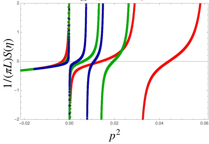
Figure 3: Predicted phase shift versus finite-volume spectrum from the Lüscher formalism for three different volumes, L = 16, 24, 32 (red, green, blue).
