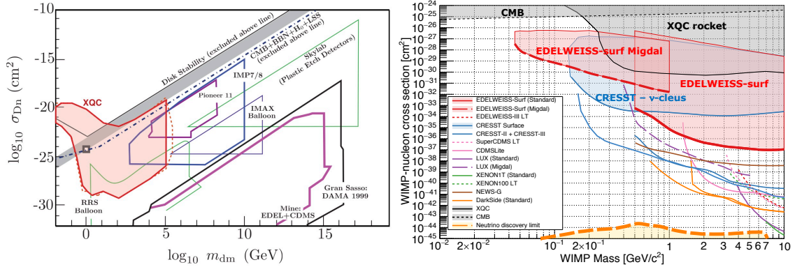
Figure 1: Left panel: constraints on large-mass SIMPs particles, taken from Ref. [10]. Right panel: experimental constraints for SIMP masses below 10 \text{ GeV}/c^2 , adapted from Ref. [14]. See references therein for the list of the different experiments appearing in the two panels.
