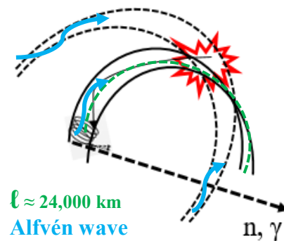
Figure 6. Schematic view of the magnetic loop. The arc length (green dotted line) is estimated as 24,000 km. Ions and electrons inside the magnetic loop repeat the back and forth motion. Alfvén wave rises up from the foot points of the magnetic loops and may collide in the center of the loops, forming the shock front.
