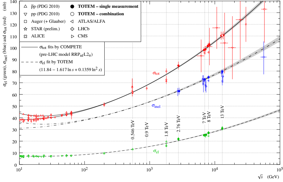
Figure 1: A compilation of total, inelastic and elastic pp cross-section measurements, see Ref. [7, 20] and references therein. The red points indicate the TOTEM total cross-section measurements at \sqrt{s} = 2.76, 7, 8 and 13 TeV. These are compared to pre-LHC models using low energy data for the extrapolation to LHC [8].
