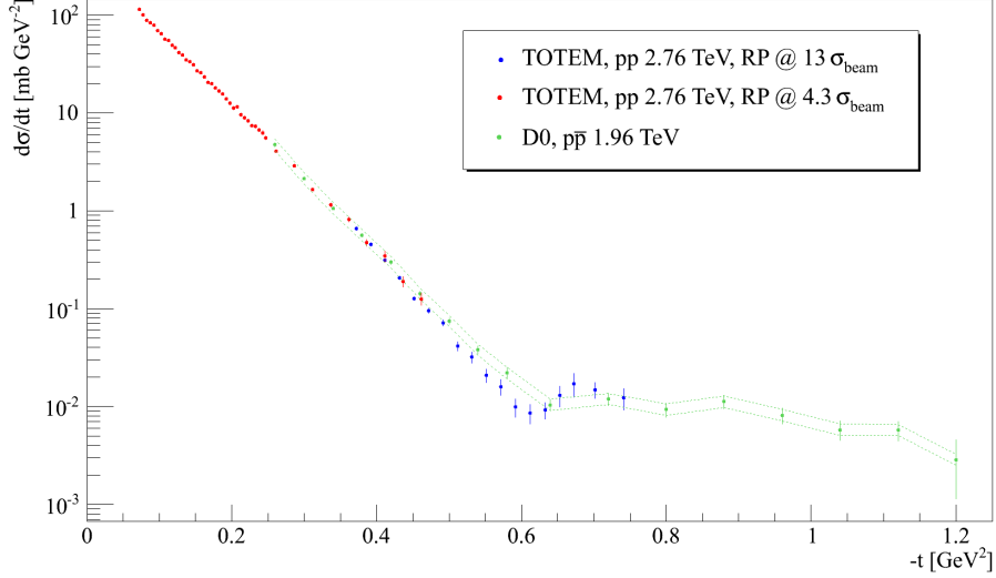
Figure 2: The differential elastic pp cross-section d\sigma/dt at \sqrt{s} = 2.76 TeV measured by the TOTEM experiment and the elastic p\bar{p} cross-section measurement of the D0 experiment at 1.96 TeV [18]. The green dashed line indicates the normalization uncertainty of the D0 measurement.
