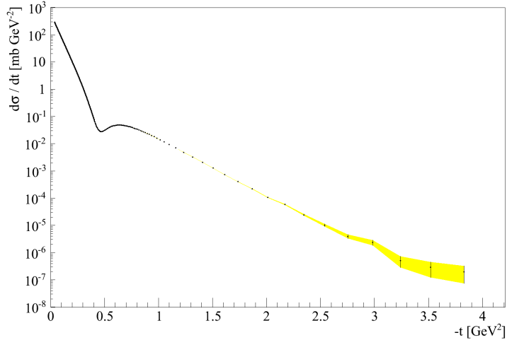
Figure 3: Differential elastic pp cross-section d\sigma/dt at \sqrt{s} = 13 TeV. The statistical and |t| -dependent correlated systematic uncertainty envelope is shown as a yellow band.
