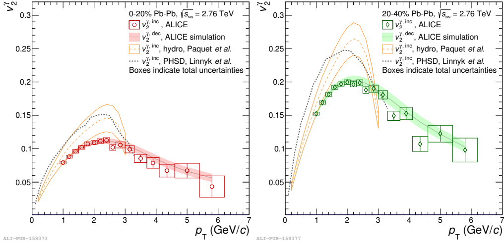
Figure 1: (Color online) The elliptic flow of inclusive and decay photons in Pb–Pb collisions at \sqrt{s_{\text{NN}}} = 2.76 TeV [2], compared to hydrodynamic [4] and transport PHSD [5] model predictions, for the 0–20% (left) and 20–40% (right) centrality classes. The boxes indicate the total uncertainty, and the vertical bars indicate the statistical uncertainty.
