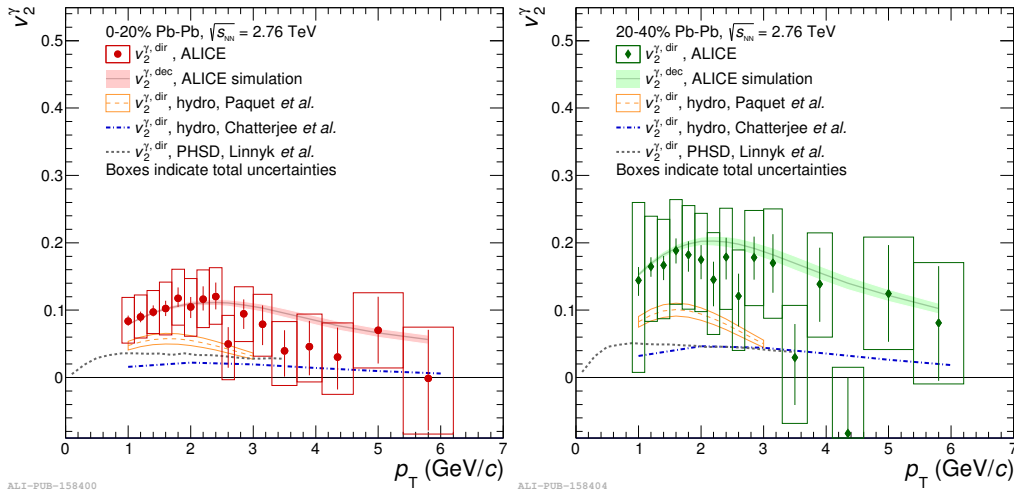
Figure 2: (Color online) The elliptic flow of direct photons in Pb-Pb collisions at \sqrt{s_{NN}} = 2.76 TeV [2], compared to hydrodynamic [4] and transport PHSD [5] model predictions in the 0–20% (left) and 20–40% (right) centrality classes. The boxes indicate the total uncertainty, and the vertical bars indicate the statistical uncertainty.
