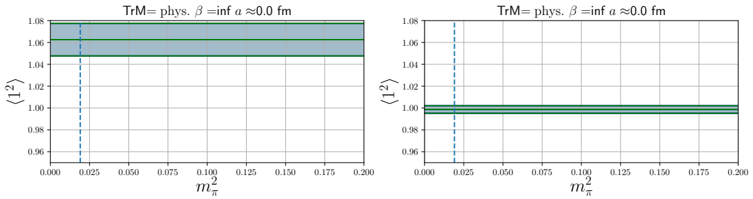
Figure 3: Continuum and chirally extrapolated value of the renormalized \mathcal{O}^+ operator Eq. (2.7) for the old and new combination of Lorentz indices in the left and right panel respectively.
