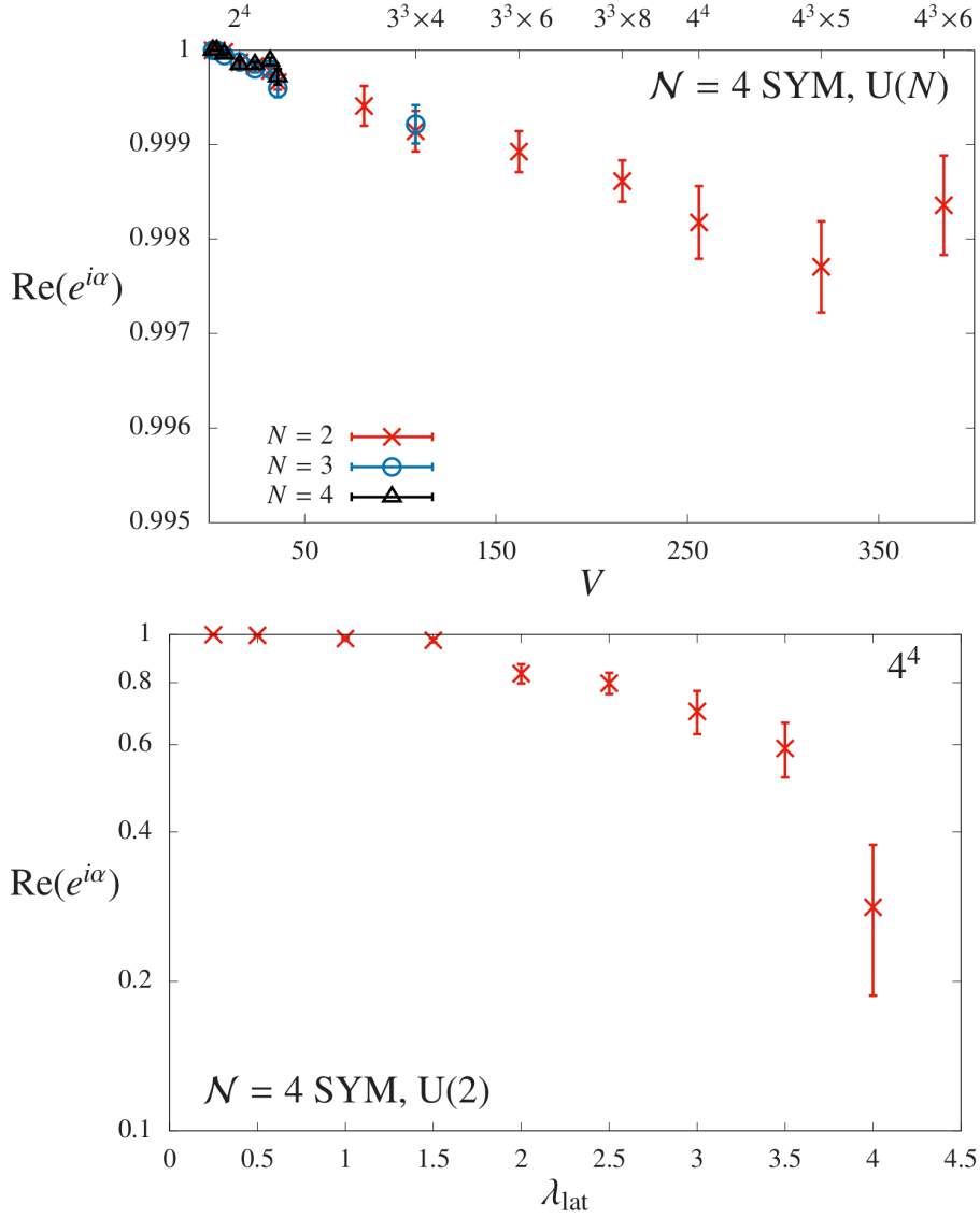
Figure 2: Results for the phase of the pfaffian \langle \text{Re}(e^{i\alpha}) \rangle_{\text{pq}} \approx \langle e^{i\alpha} \rangle_{\text{pq}} from lattice \mathcal{N} = 4 SYM in four dimensions. Top: With fixed 't Hooft coupling \lambda_{\text{lat}} = 0.5 , only per-mille-level fluctuations are observed for U(N) gauge groups with N = 2, 3 and 4 , up to the largest accessible volumes. Adapted from Ref. [123]. Bottom: On a fixed 4^4 lattice volume, the phase fluctuations increase significantly for stronger couplings \lambda_{\text{lat}} \gtrsim 2 , obstructing studies of \lambda_{\text{lat}} \gtrsim 4 with this lattice action. Adapted from Ref. [161].
