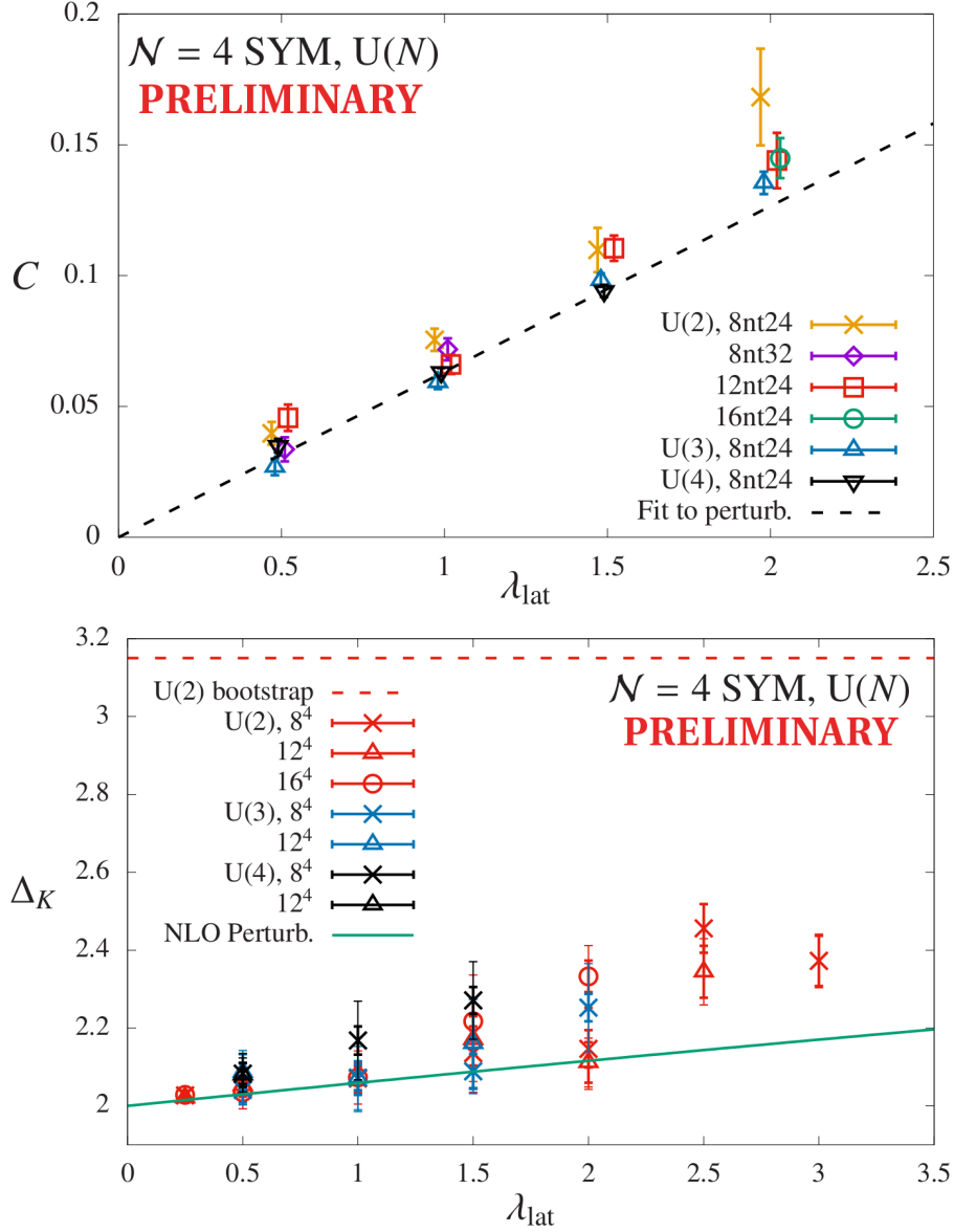
Figure 1: Preliminary results from ongoing 4d lattice \mathcal{N} = 4 SYM calculations with gauge groups U(2), U(3) and U(4). Top: The static potential Coulomb coefficient, from L^3 \times N_t lattices with L \leq 16 and N_t \leq 32 , appears consistent with leading-order perturbation theory (black dashed line) for \lambda_{\text{lat}} \leq 2 . Bottom: The Konishi scaling dimension, from MCRG stability matrix analyses of L^4 lattices with L \leq 16 , also appears consistent with perturbation theory (and well below bootstrap bounds) for \lambda_{\text{lat}} \lesssim 3 .
