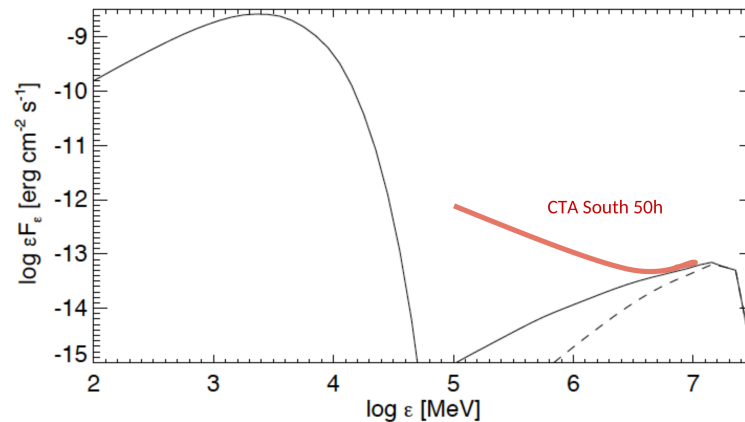
Figure 7: The CR and ICS components. For the ICS: continuous – soft photon field optical to far-IR dashed – soft photon field optical to near-IR.
