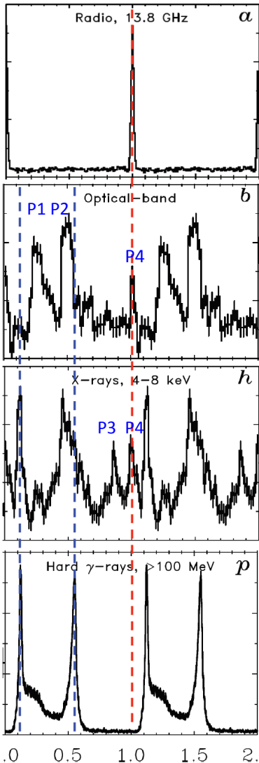
Fig.1 – The Vela lightcurves at radio, optical, hard X-rays and \gamma -rays (from [5]).
