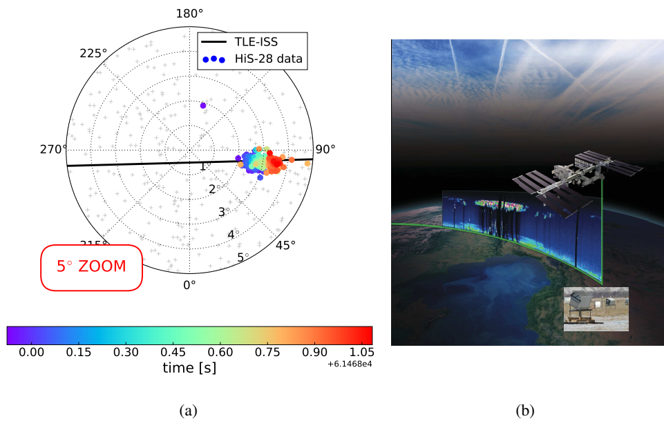
Figure 1: (a) Example of an observed ISS-passage (2017/03/25), color code gives time evolution within \sim 1 sec. Grey crosses illustrate the reconstructed EAS directions, as recorded \pm 5 min around the ISS passage. (b) The Cloud Aerosol Transport System (CATS) operating from the ISS, with a LIDAR scanning the atmosphere profile (adapted from [11]).
