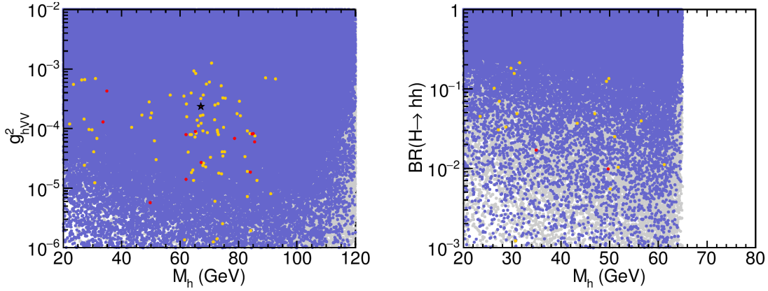
Figure 3: g_{hVV}^2 (relative to the SM value) (left) and BR(H \rightarrow hh) as a function of M_h (right) in the heavy Higgs case. The color coding is as in Fig. 1.
