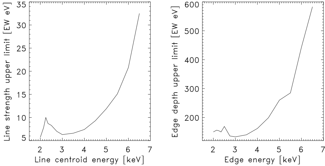
Figure 5: Upper limit to the equivalent width of absorption lines (left) and absorption edges (right) as a function of line centroid energy and edge energy, respectively. These values are based on the total burst spectrum from all -1 and +1st orders of HEG and MEG.
