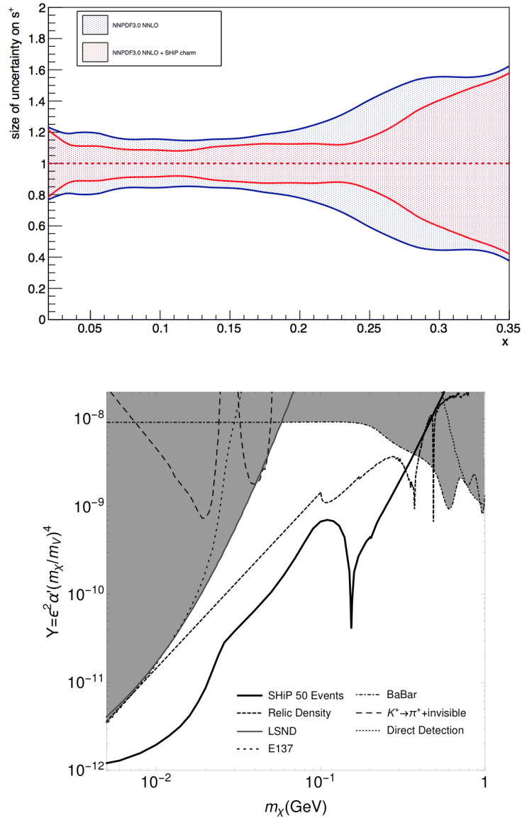
Figure 3: Top: improvement of the accuracy on s^+ with SHiP (red) compared to the present status (blue) in the 0.02 < x < 0.35 range. Bottom: sensitivity to the dark matter in the assumption that m_\chi/m_A = 1/5 .
