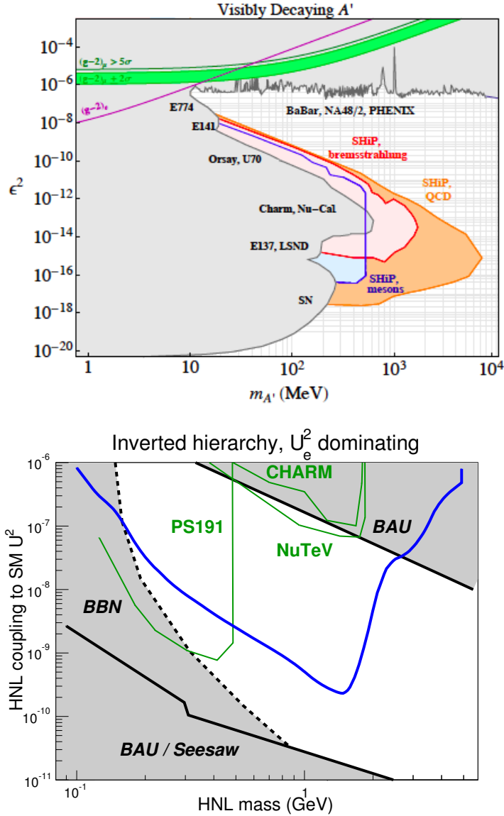
Figure 2: Top: exclusion limit at 90% C.L. in the dark photon search, in the plane defined by its mass and \epsilon^2 squared coupling. Bottom: exclusion limits at 90% C.L. in the heavy neutral lepton search, for inverted hierarchy with U_e^2 dominating, according to Ref. [11].
