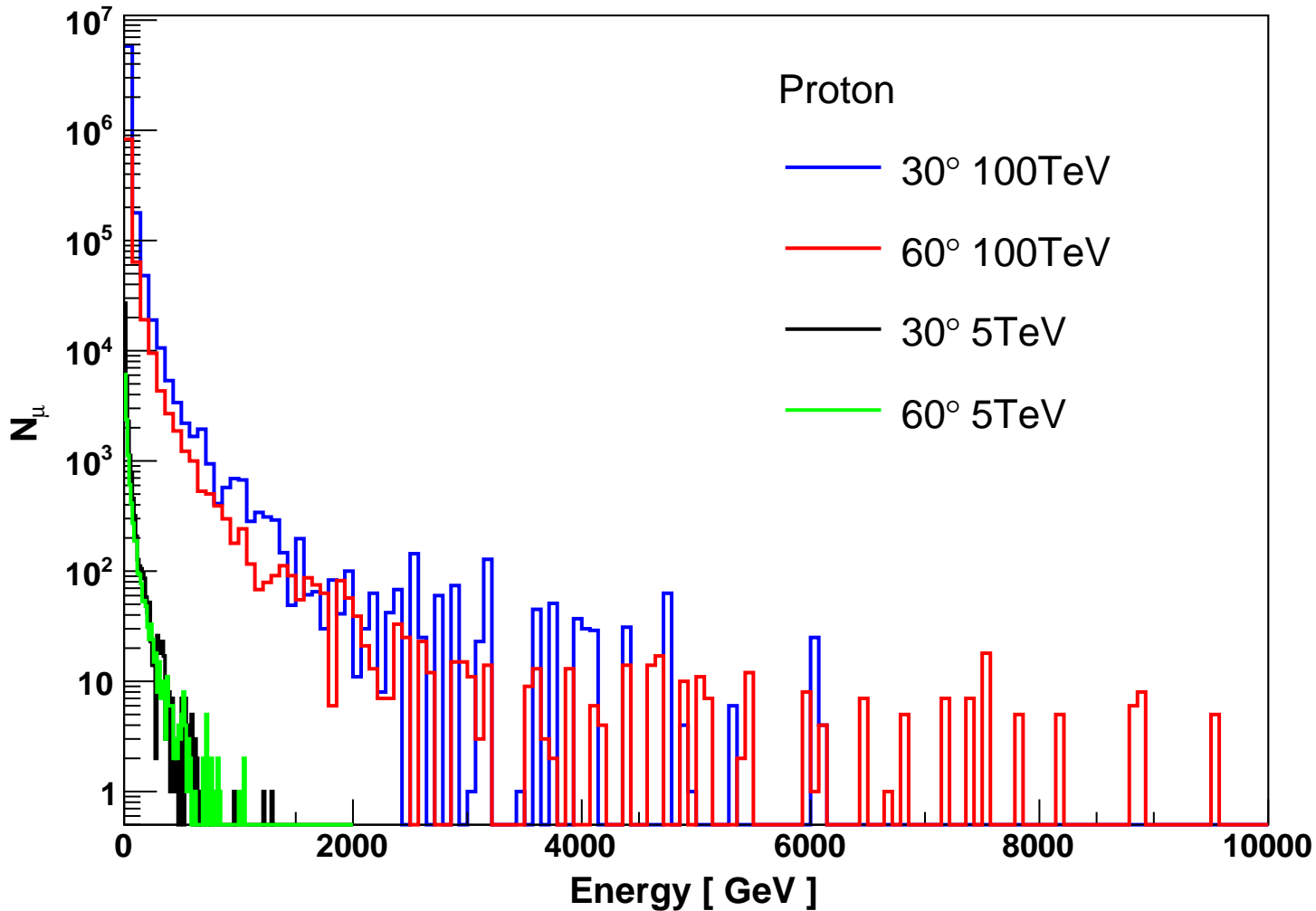
Energy distribution of \mu^\pm for each zenith angle
