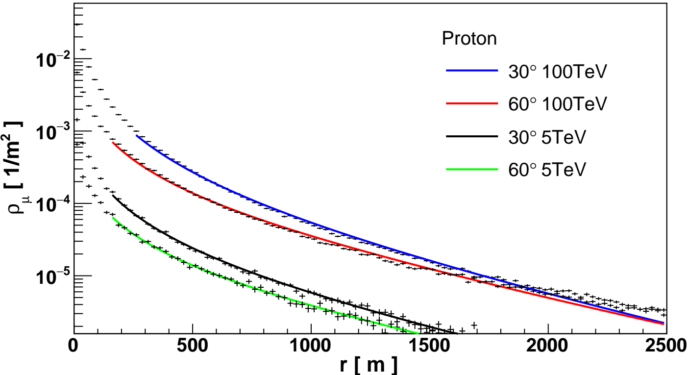
Lateral average distribution of \mu^\pm and fit
