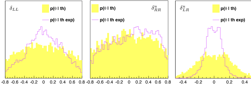
Figure 2: Prior (yellow) and posterior (purple) probability distributions of three selected flavour-violating parameters of our NMFV-MSSM setup.
