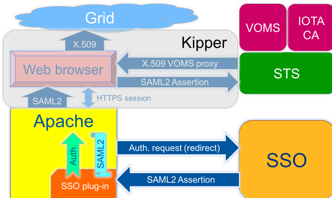
Fig. 3. Kipper workflow.
