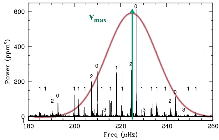
Figure 7: Oscillation power spectrum with a typical Gaussian-like shape for the red giant star KIC 4448777 observed by Kepler . The harmonic degrees of the modes ( l = 0, 1, 2, 3 ) and \nu_{max} the frequency of maximum oscillation power are indicated.
