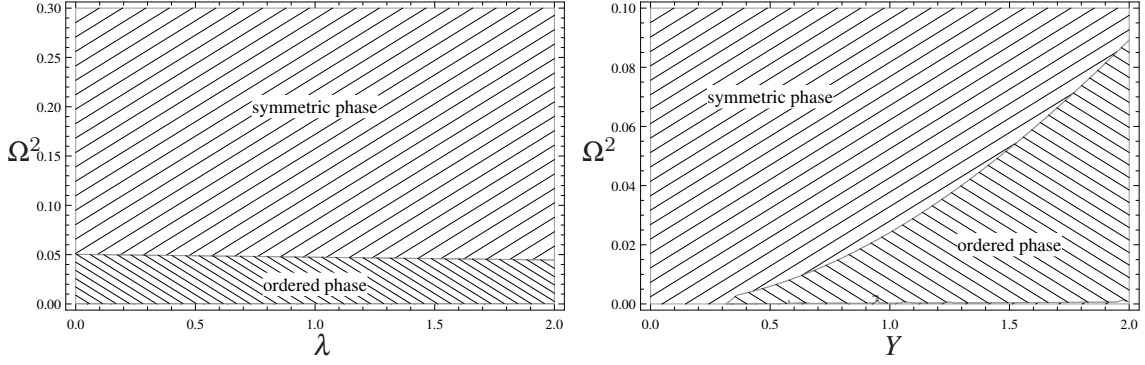
(a) The subspace of the phase space given by the Eq. Y = 1.461 .
