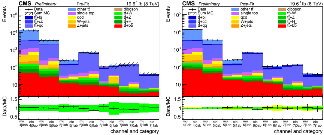
Figure 1: The event yields per category before(left) and after(right) the fit are shown. The green and yellow bands represents the one and two sigma standard deviations of the statistical and systematic uncertainties.
