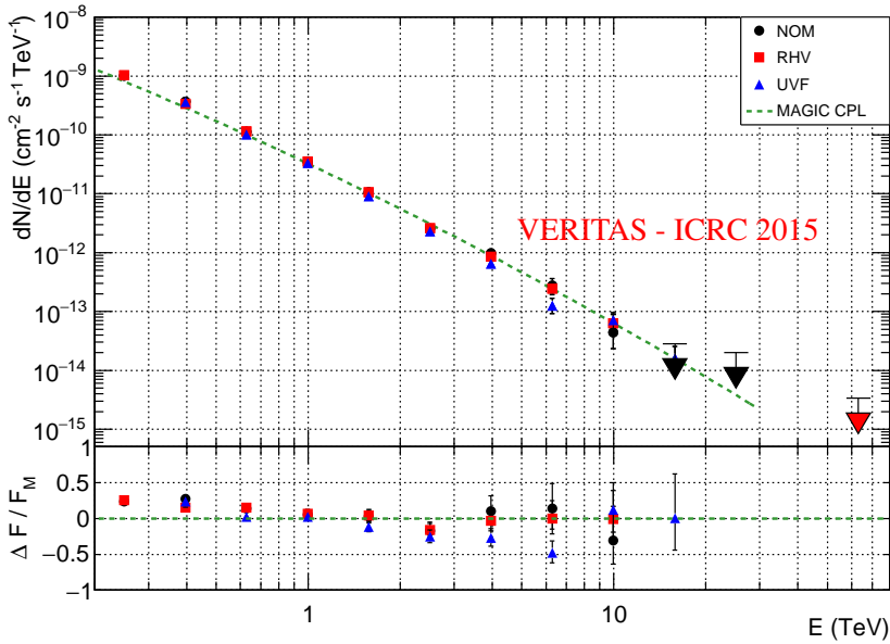
Figure 6: Top: Crab nebula spectra resulting from the NOM, RHV, and UVF data sets. The curved power law from [18] is also indicated. The upper limits are at the 95% confidence level. Bottom: Residuals of the three data sets from the curved power law from [18]. The upper limits have intentionally been omitted for clarity.
