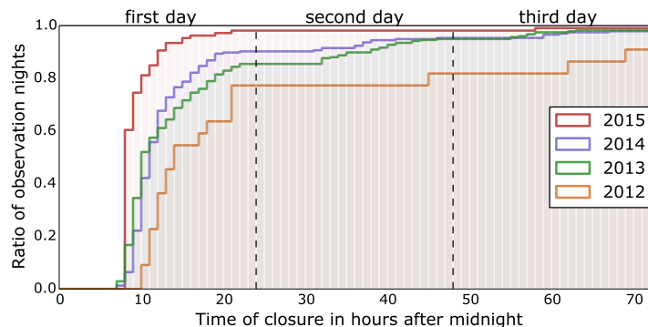
Figure 3: OSA performance for closing M1 for the last 4 years of operation. The y-axis shows the ratio of nights closed before x hours after midnight. Statistics could only be gathered from 2012 on.
