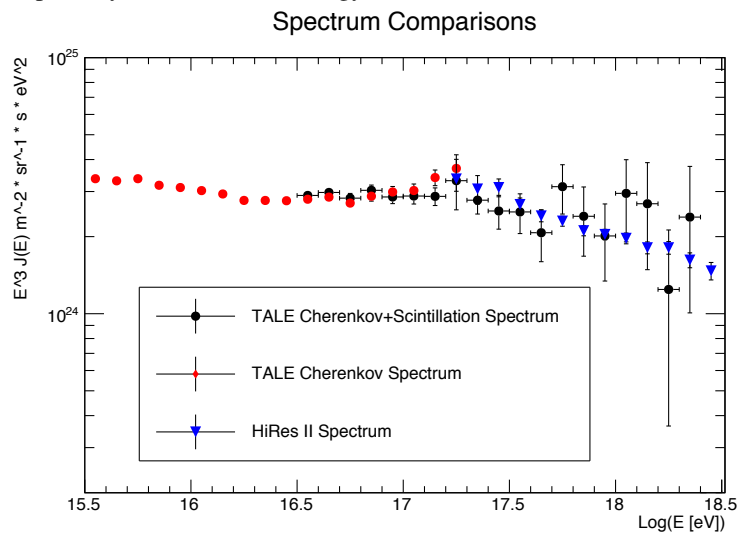
Figure 8: The measured flux of cosmic rays by the TALE FD in this analysis is shown in black. The flux of cosmic rays using only Cherenkov dominant events performed by Tareq AbuZayad is shown in red. The previous measurement of the spectrum reported by the HiRes experiment is shown in blue. Note that the flux has been multiplied by the cube of the energy in order to enhance the features of the spectrum.
