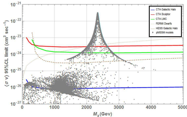
Figure 4. Zoomed sensitivities in the TeV mass range together with pMSSM models extracted from [25].
