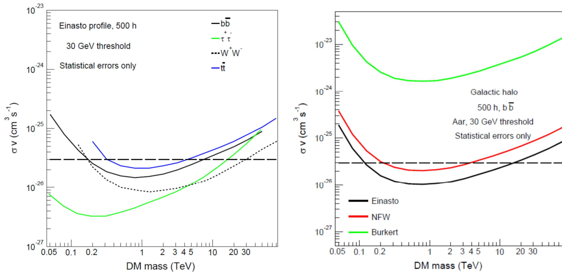
Figure 1. Left: Sensitivity for \sigma v from observation on the Galactic Halo with Einasto dark matter profile and for different annihilation modes as indicated. Right: for cuspy (NFW, Einasto) and cored (Burkert) dark matter halo profiles. For both plots only statistical errors are taken into account. The dashed horizontal lines indicate the level of the thermal cross-section of 3 \times 10^{-26} \text{ cm}^3 \text{ s}^{-1} .
