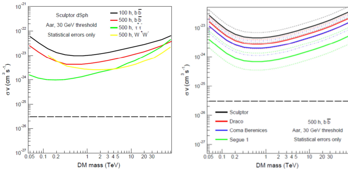
Figure 2. Left: Sensitivity for \sigma v from observation on the classical dwarf galaxy Sculptor for different annihilation modes as indicated. Right: Sensitivity for 500 h observation on the classical dSphs Draco and Sculptor, and the ultra-faint dwarf galaxies Segue 1 and Coma Berenices as indicated. Dashed lines correspond to \pm 1\sigma on the J-factors. Sensitivity is computed assuming the b\bar{b} annihilation mode and statistical errors only are taken into account.
