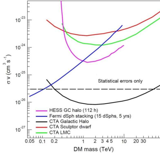
Figure 3. Comparison of predicted sensitivities in \sigma v for the targets of: the Milky Way Halo; the Large Magellanic Cloud and the dwarf galaxy Sculptor. The CTA sensitivity curves use the same method and W^+W^- annihilation modes for each target and the NFW dark matter profile. The sensitivity calculations have a 30 GeV threshold for the MW and Sculptor and 200 GeV for the LMC. The sensitivities for the three targets are all for 500 hours taking into account only statistics errors; for the MW and the LMC, the systematics of backgrounds must be very well controlled to achieve this statistically possible sensitivity. The comparisons with the H.E.S.S. and Fermi-LAT results come from [13] and [24] respectively.
