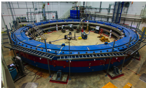
Figure 4: The g-2 storage-ring magnet at Fermilab with a yoke assembly completed (Image credit: Fermilab.)
