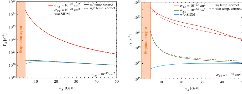
Figure 2: Total annihilation rate \Gamma_A for \sigma_{\chi p} = 10^{-45} \text{ cm}^2 and 10^{-47} \text{ cm}^2 with \sigma_{\chi\chi} = 10^{-23} \text{ cm}^2 and 10^{-24} \text{ cm}^2 . Dashed lines are those results calculated with T_\chi = T_c .
