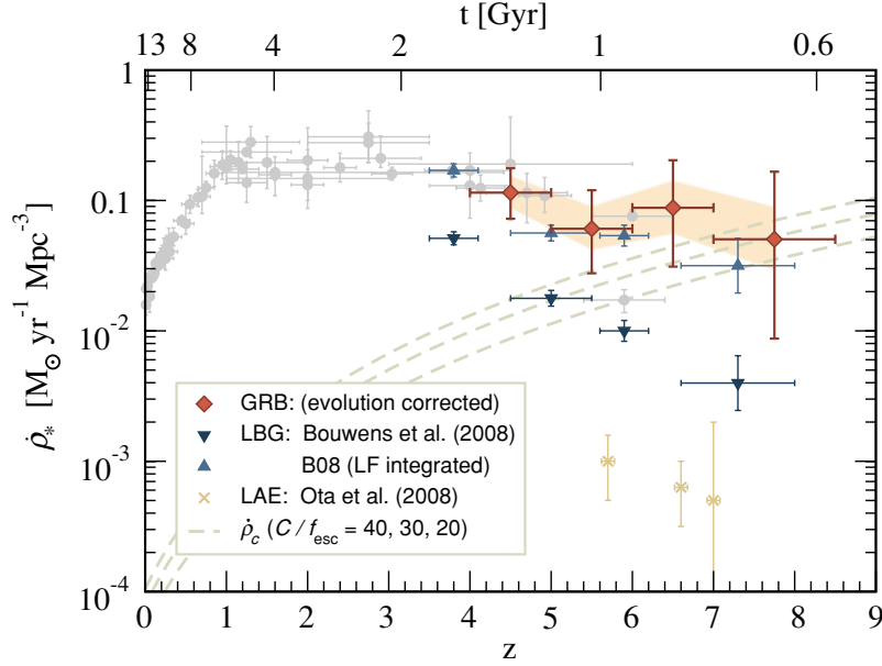
Figure 5: The cosmic star formation rate (SFR) history (Kistler et al. 2009), with data from several sources (Hopkins & Beacom 2006, Bouwens et al. 2008, Ota et al. 2008). The rates inferred from high- z GRBs are shown as diamonds. The three dashed curves (Madau et al. 1999) give the critical SFR \dot{\rho}_c required to balance recombination, for C/f_{\text{esc}} = 40, 30, 20 (top to bottom), where C is the clumpiness of the intergalactic medium and f_{\text{esc}} the fraction of photons that escape their galaxy.
