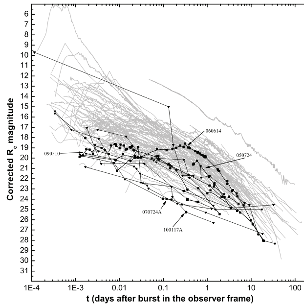
Figure 3: R-band afterglow light curves, corrected for Galactic extinction and host galaxy contribution, of Type I (black lines and points) and Type II (thin gray lines) GRBs (Kann et al. 2011). These types correspond closely to short and long GRBs, respectively. In general the optical afterglows are fainter for short GRBs.
