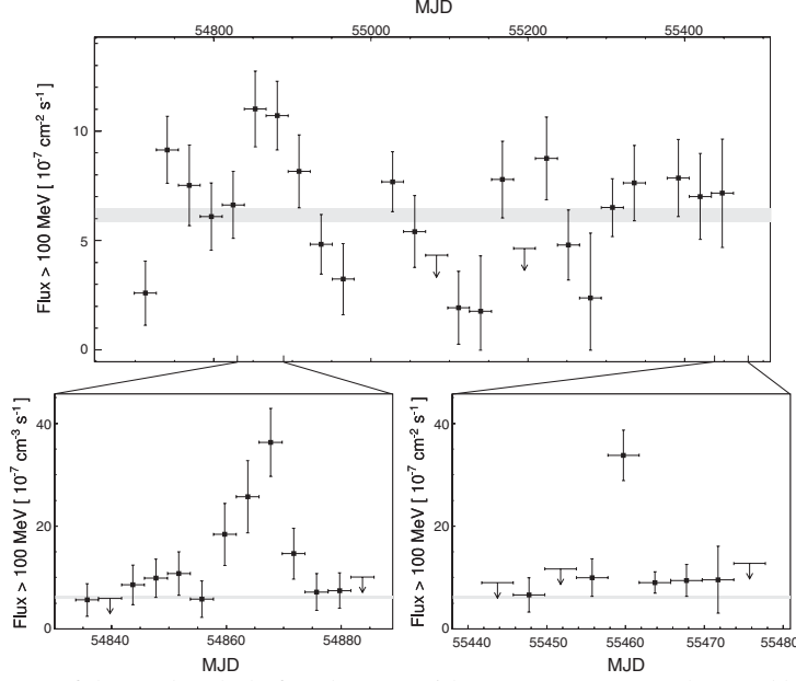
Figure 1: A light curve of the Crab nebula for photons with E > 100 MeV as observed by Fermi /LAT (Abdo et al. 2011).
