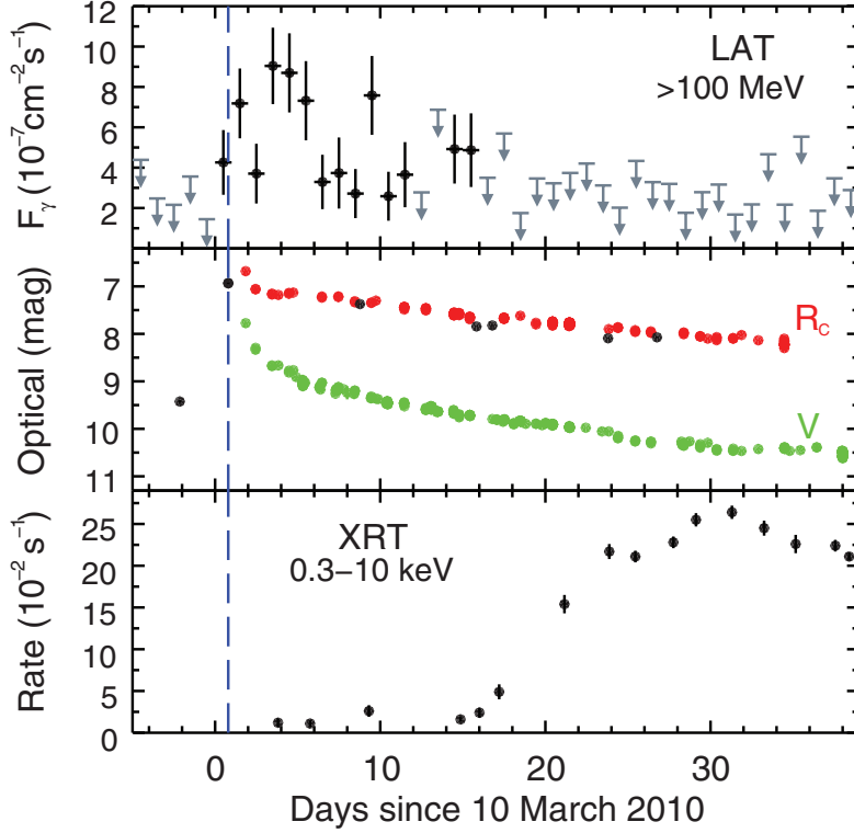
Figure 2: Light curves of V407 Cyg in \gamma -rays (Abdo et al. 2010) from Fermi /LAT ( upper panel ), optical ( middle panel ), and X-rays as seen by Swift /XRT ( bottom panel ). Vertical dashed blue line indicates the time of the optical nova. The \gamma -rays peak 3 to 4 d later.
