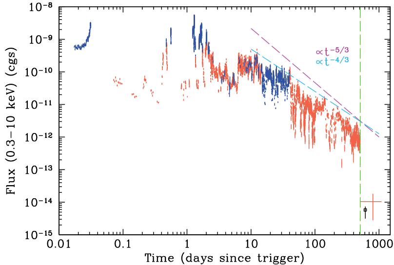
Figure 6: The long term XRT light curve for Swift 1644, the jetted tidal disruption event (Mangano et al. 2014). The decay closely follows -4/3 ; a decay -5/3 is disfavored.
