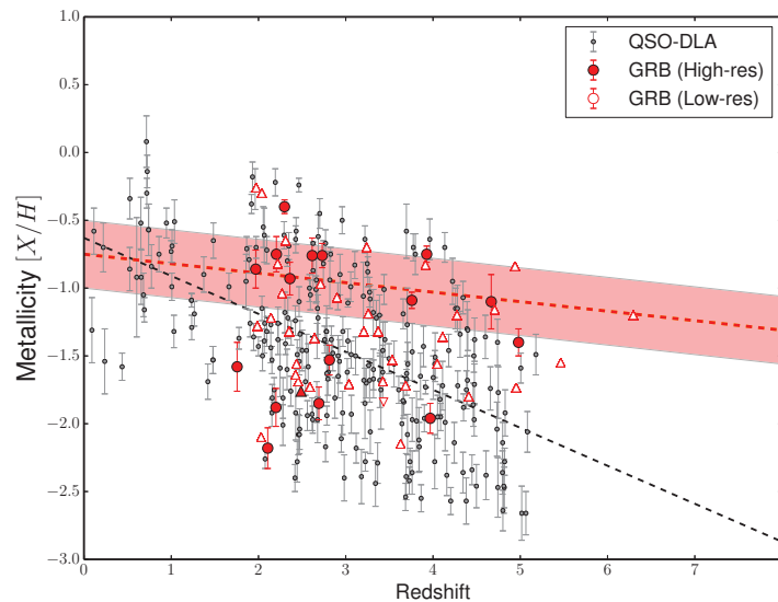
Figure 4: Metallicity versus redshift for QSO-DLA and GRBs (Cucchiara et al. 2014).
