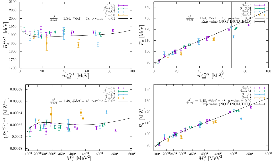
Figure 11: LO+NLO+NNLO fit in x expansion (top) or \xi expansion (bottom) of M_\pi^2/m_{ud} or m_{ud}/M_\pi^2 (left) and F_\pi (right) versus m_{ud} or M_\pi^2 , respectively.
