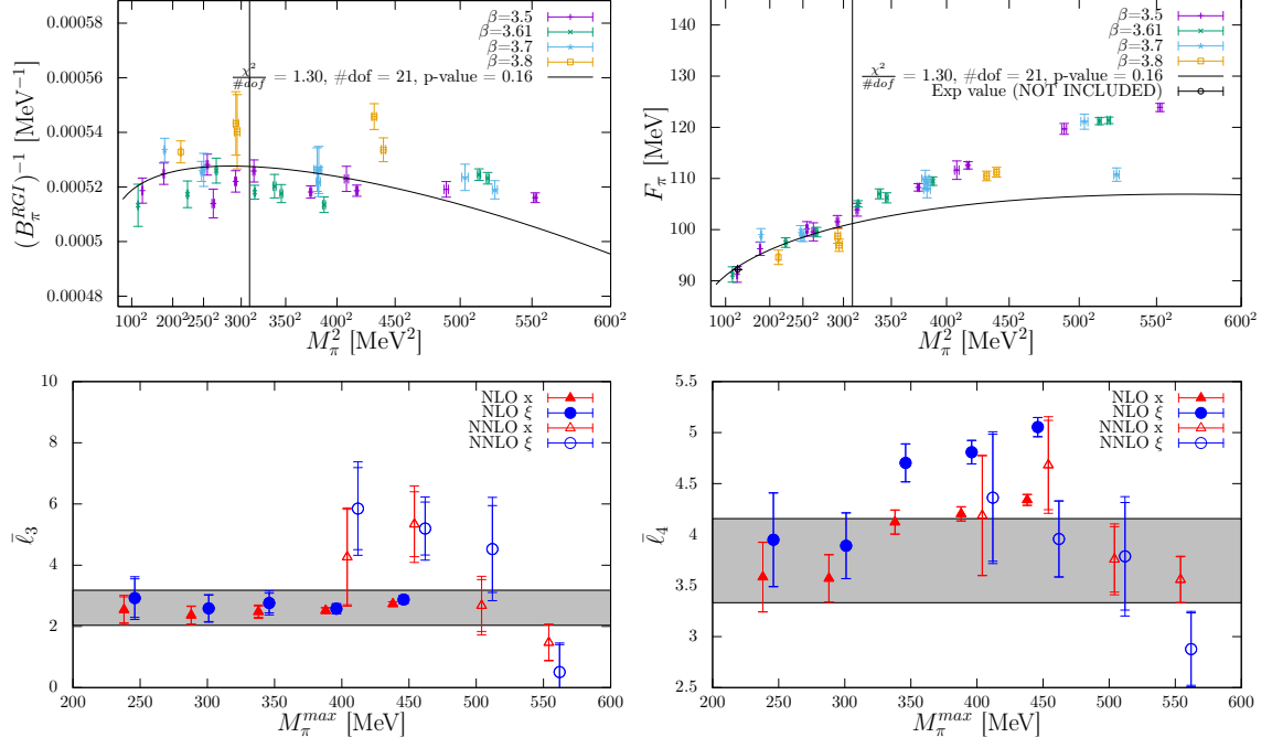
Figure 10: Top: \xi expansion fit at NLO of m_{ud}/M_\pi^2 and F_\pi versus M_\pi^2 with M_\pi^{\max} = 300 MeV. Bottom: fit parameters \bar{\ell}_3, \bar{\ell}_4 as a function of M_\pi^{\max} .
