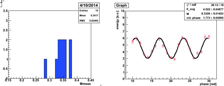
Fig 4: M measured by fringe scans in the 174^\circ mode. (left) :10 continuous scans resulted in M_{\text{meas}} = 0.341 \pm 0.025 (stat.). Without taking into account of systematic errors of Shintake Monitor, this corresponds to \sigma_{y,\text{meas}} = 61.9 \pm 2.1 \text{ nm} . (stat.) (right) : one scan from this set : M_{\text{meas}} \sim 0.33 , \sigma_{y,\text{meas}} \sim 63 \text{ nm} . Plotted here are the average and S.D, of 10 pulses used for measurement at each phase.
