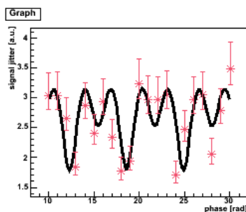
Fig 6 : \Delta\phi for an example 174^\circ mode N_{av}=50 scan is estimated as 0.74\pm 0.03 rad, corresponds to \Delta y = 31\pm 1 nm
