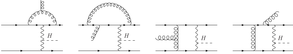
Figure 1: A representative selection of one-loop Feynman diagram topologies for EW Hjjj production.
