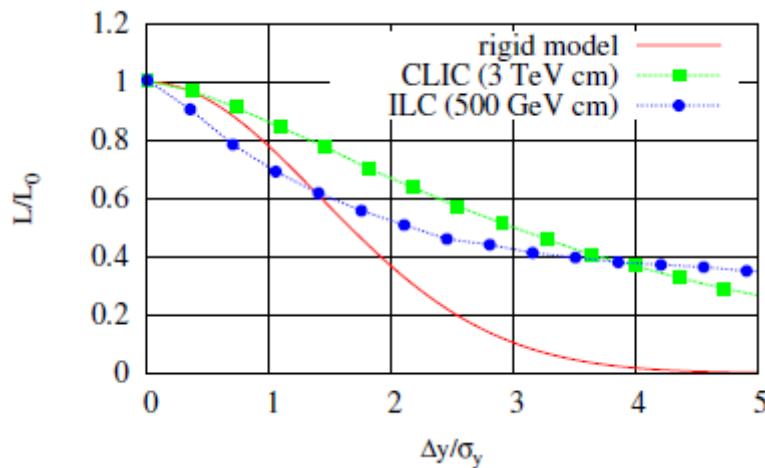
Figure 1: Luminosity relative to design vs. relative vertical beam-beam position offset at the IP.
