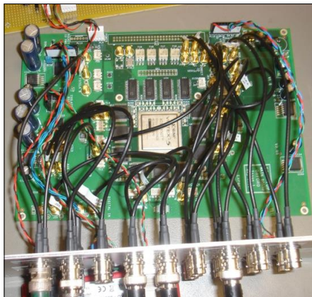
Figure 6: FONT5 digital feedback board.
