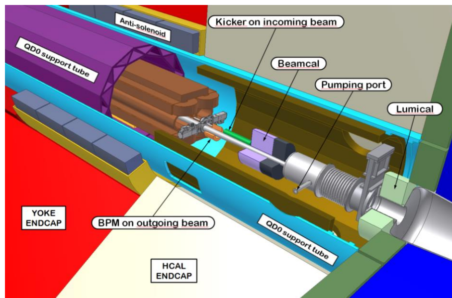
Figure 3: Layout of IP intra-train feedback system components in the CLIC interaction region [7].
