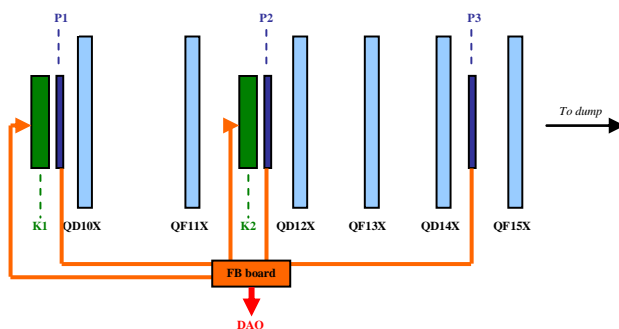
Figure 5: Schematic of FONT5 at the ATF2 extraction beamline showing the relative locations of the kickers, BPMs and the elements of the feedback system.
