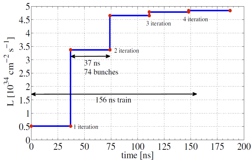
Figure 4: Luminosity vs. time for a simulated bunchtrain crossing at CLIC.
