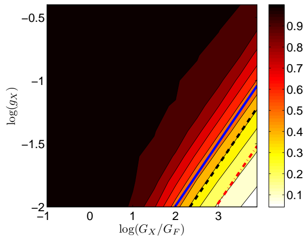
Figure 1: Contours of equal thermalization of the sterile neutrino. \Delta N_\nu is given by the colors. The solid, dashed, and dot-dashed lines correspond to hidden bosons with masses M_X = 300, 200, and 100 MeV respectively (reproduced from [4]).
