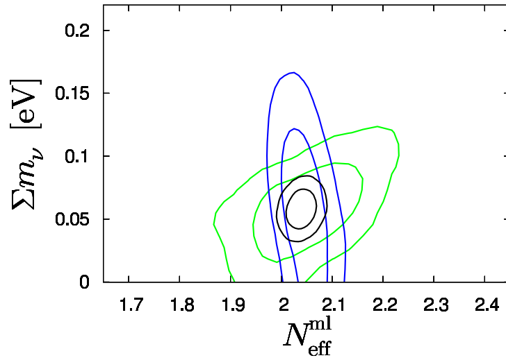
Figure 2: Marginalised joint two-dimensional 68% and 95% credible contours for \Sigma m_\nu and the effective number of massless neutrinos from the EUCLID-like survey forecast performed in [8]. The different contours are for Planck CMB data + a EUCLID-like cluster data set (blue), Planck CMB data + a EUCLID-like photometric shear and galaxy survey (green), and all data sets combined (black) (Reproduced from [8]).
