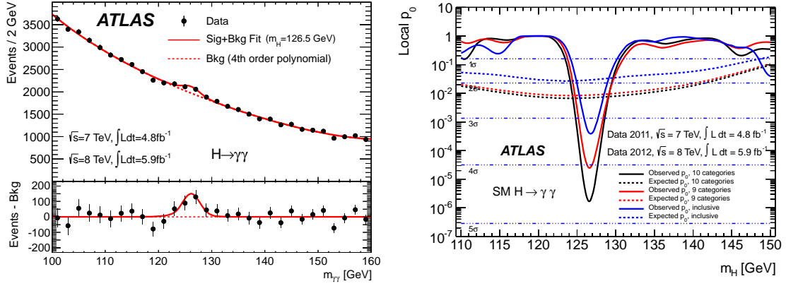
Figure 1: [Left] Invariant mass distribution for the combined \sqrt{s} = 7 TeV and \sqrt{s} = 8 TeV data samples. Superimposed is the result of a fit including a signal component fixed to a hypothesized mass of 126.5 GeV and a background component described by a fourth-order Bernstein polynomial. The bottom inset displays the residual of the data with respect to the fitted background [1]. [Right] Expected and observed local p_0 for the analysis using 10 categories, compared to an analysis using only 9 categories (no 2-jets category) and a fully inclusive analysis for the combined \sqrt{s} = 7 TeV and \sqrt{s} = 8 TeV data [1].
