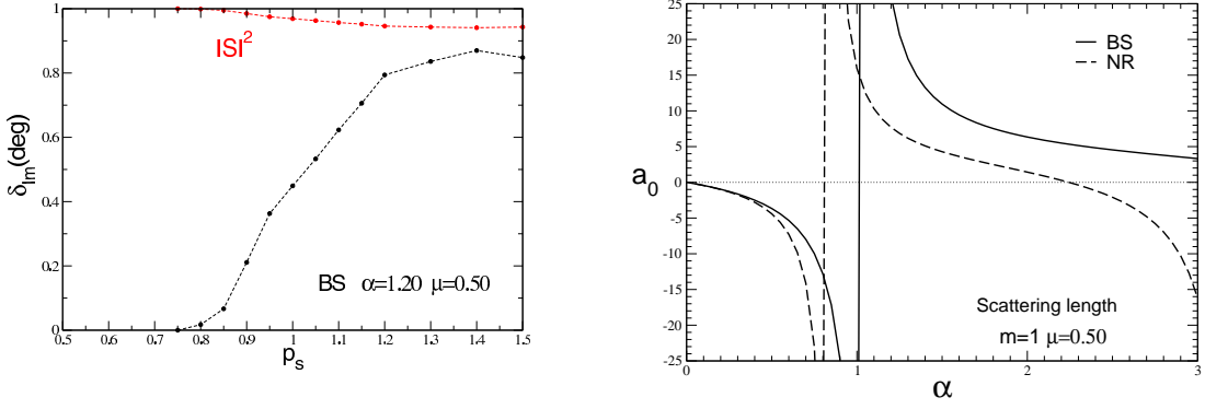
Figure 2: Left panel: imaginary part of the phase shift (solid) and squared modulus of the S-matrix (dashed). Right panel: scattering length vs. \alpha for \mu = 0.5 calculated via BS (solid) and Schrödinger equations (dashed).
