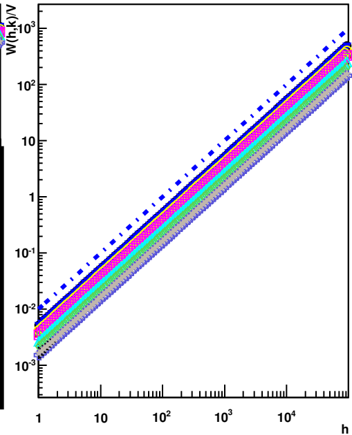
Free energy at large h values
