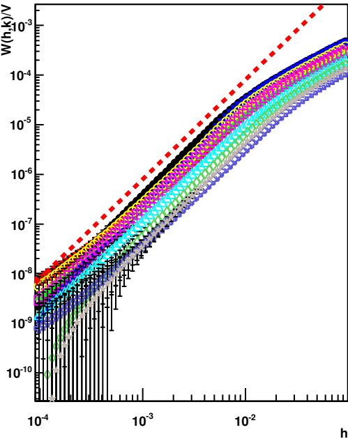
Free energy at small h values
