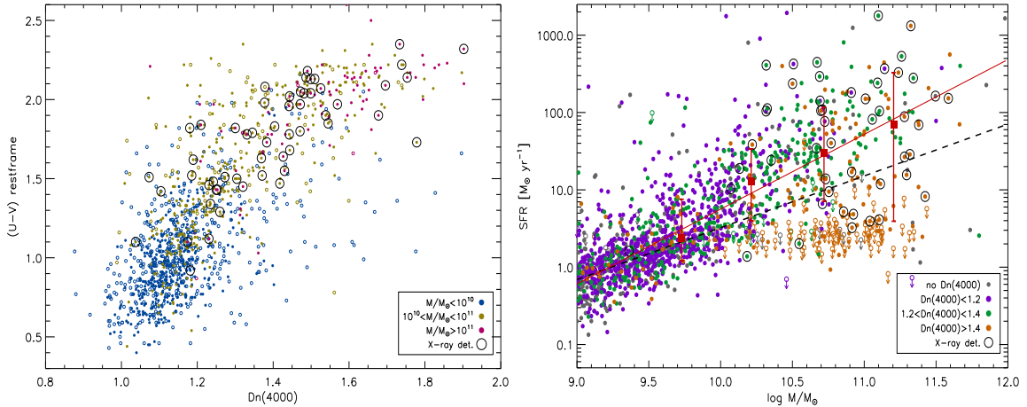
Figure 2: (Left): U-V vs D_n(4000) with color coding for stellar mass. Symbols as in Fig. 1. (Right): SFR estimate from the UV+IR emission vs stellar mass with color coding for the D_n(4000) index. Sources detected (undetected) at 24 \mu\text{m} are shown with solid (open) symbols. Big squares represent average values for sources with SFR estimates (no upper limits) in bins 0.5 dex wide and the solid line is the best linear fit of \log(\text{SFR}) vs \log(M_*) . For reference, the 'main sequence' from [8] is shown in dashed line.
