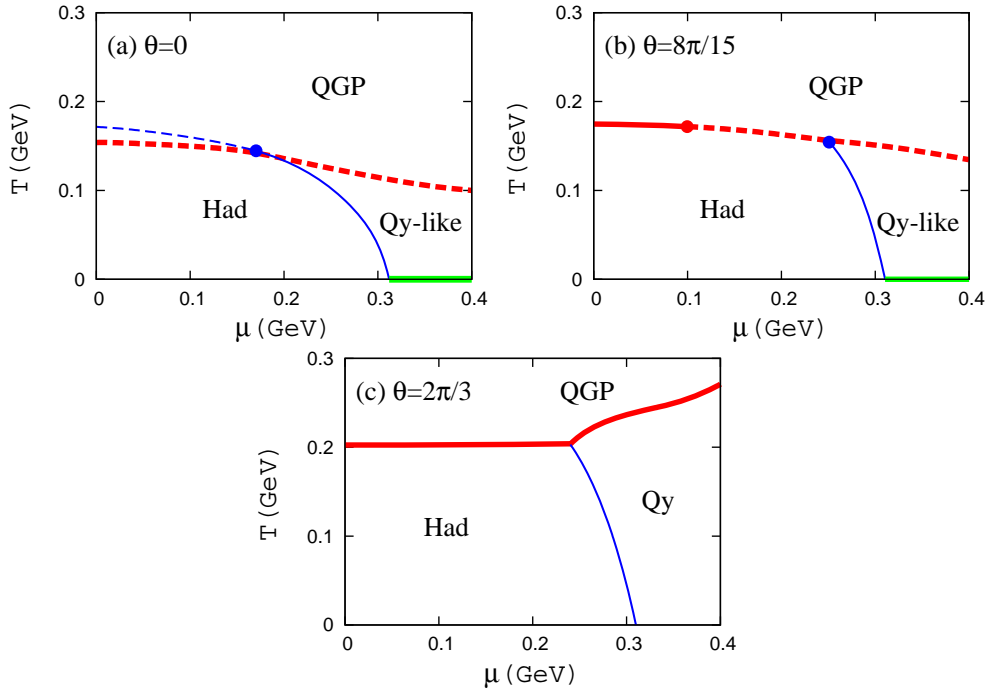
Figure 3: Phase diagram in the \mu - T plane. Panels (a)-(c) correspond to three cases of \theta = 0, 8\pi/15 and 2\pi/3 , respectively. The thick (thin) solid curve means the first-order deconfinement (chiral) phase transition line, while the thick (thin) dashed curve does the deconfinement (chiral) crossover line. The closed circles stand for the endpoints of the first-order deconfinement and chiral phase transition lines. In panels (a) and (b), the thick-solid line at T = 0 and \mu \gtrsim M_f = 323 MeV represents the quarkyonic phase.
