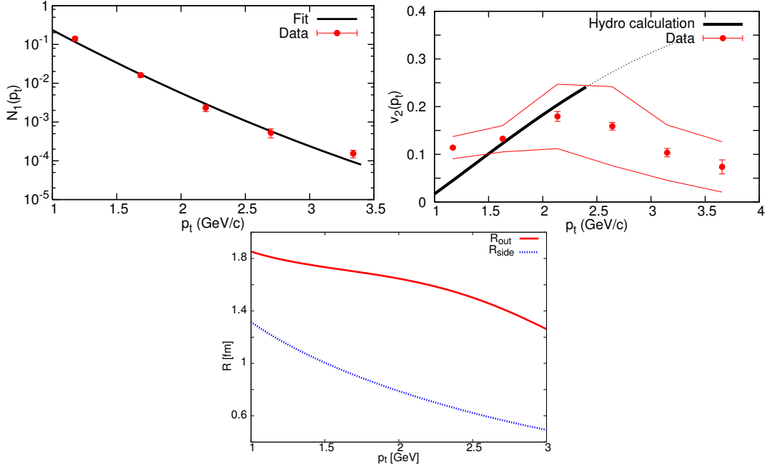
Figure 2: Fit to direct photon invariant transverse momentum data [6] (top left), comparison to elliptic flow data [11] (top right) and direct photon HBT predictions (bottom). See the model parameters in Table 1.
