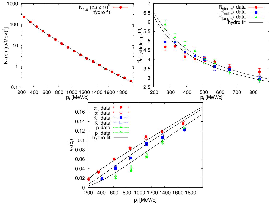
Figure 1: Fits to invariant momentum distribution of pions [8] (top left), HBT radii [10] (top right) and elliptic flow [9] (bottom). See the obtained parameters in Table 1. In the middle plot the lower curve is the fit to R_{\text{out}} and R_{\text{side}} .
