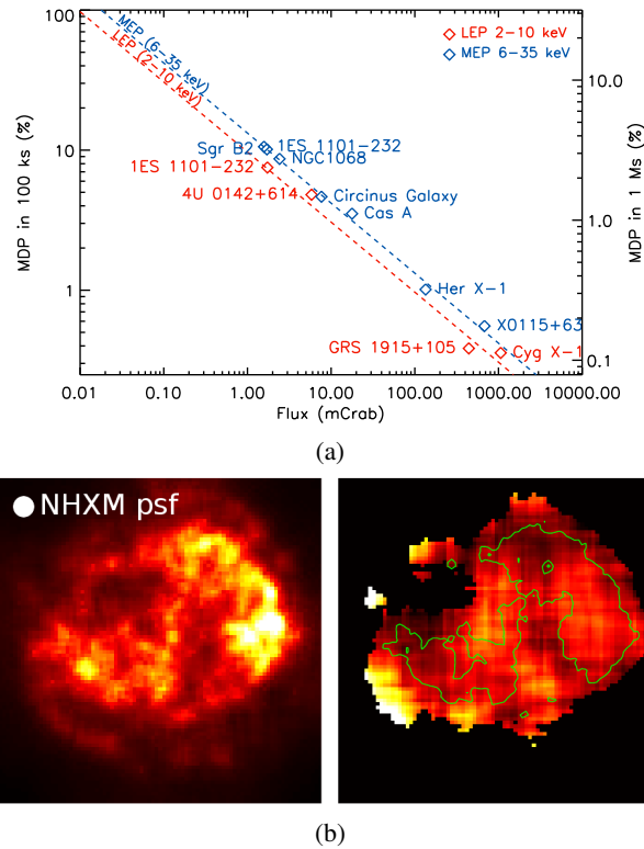
Figure 2: (a) Minimum detectable polarization (at the 99% confidence level) for the LEP and the MEP. The dashed lines refer to sources with a Crab-like spectrum. Sources with harder or softer spectra locate below and above the lines. The sensitivity for bright sources will allow for phase or energy resolved polarimetry at 1-2% level. (b) Cas A as imaged by XMM between 8.10 and 15 keV (left) and hardness ratio (right) [13]. Superimposed is the NHXM MEP point spread function. The field of view is sufficient to image all the source with a single pointing.
